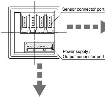
Power supply / Output connector (8P)
